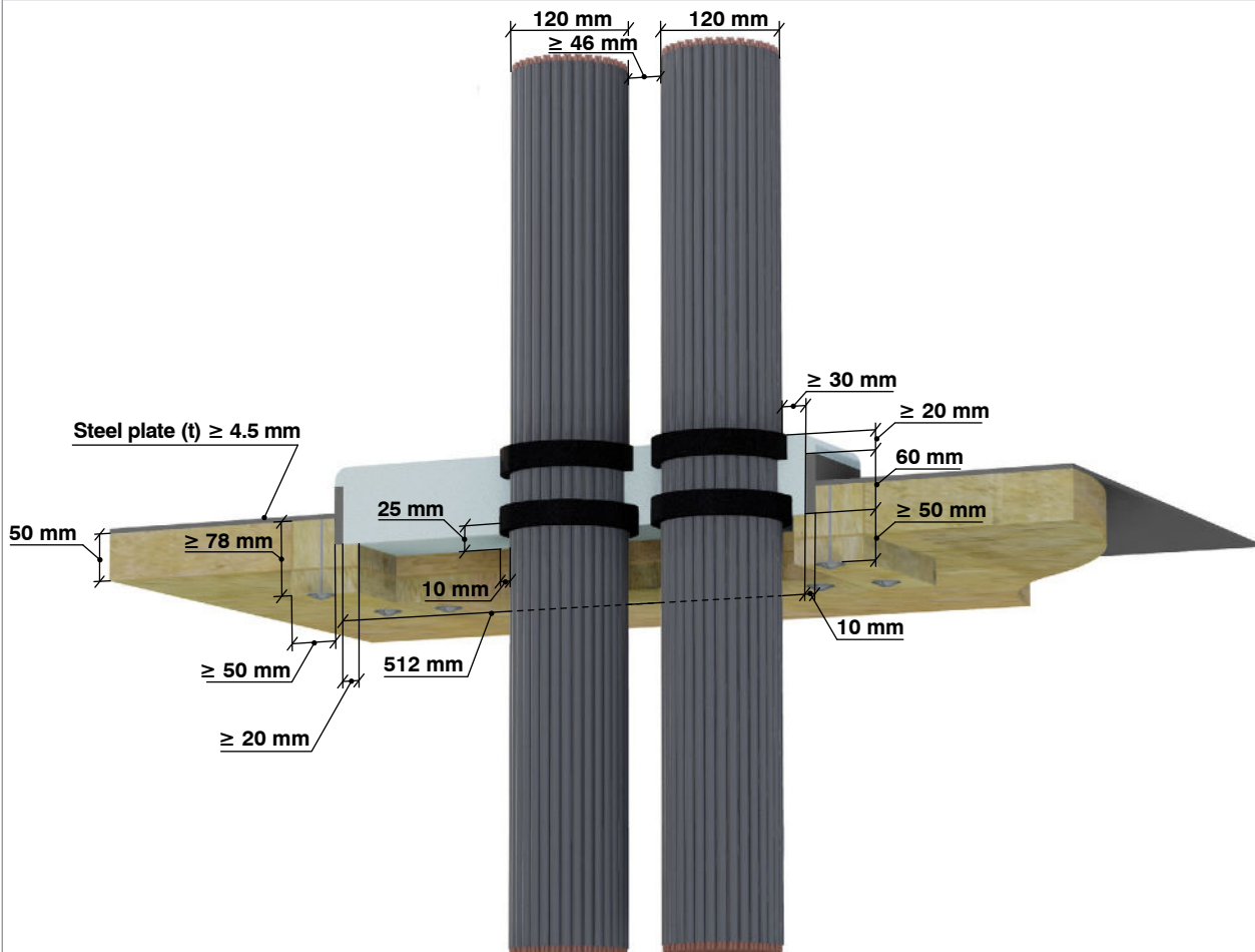
Figure 13. Thickness of GPGM 80 mm in 60 mm sleeve
