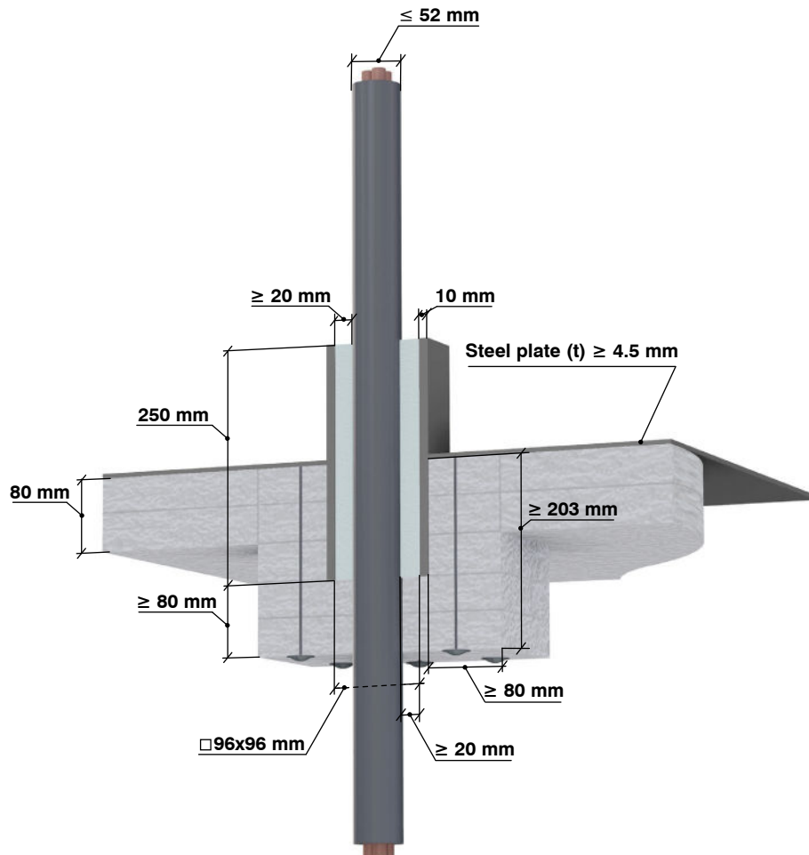
Figure 22. Thickness of GPGM 250 mm in 250 mm sleeve
