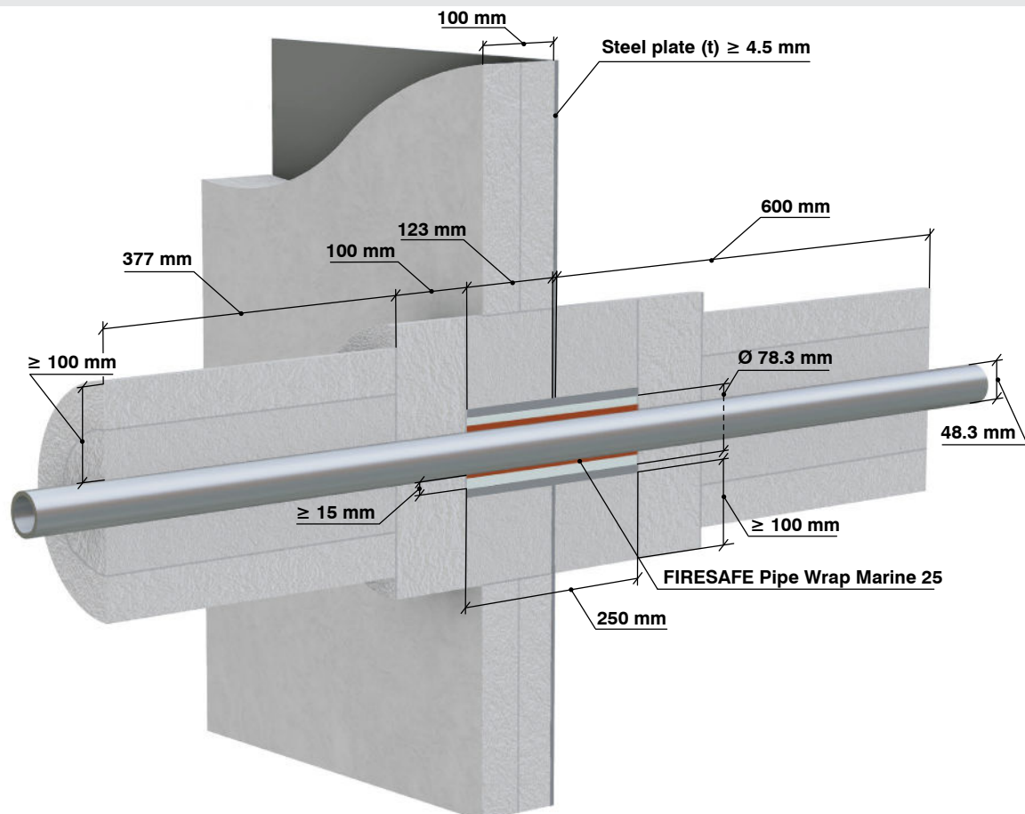
Figure 10. Thickness of GPGM 250 mm in 250 mm sleeve
