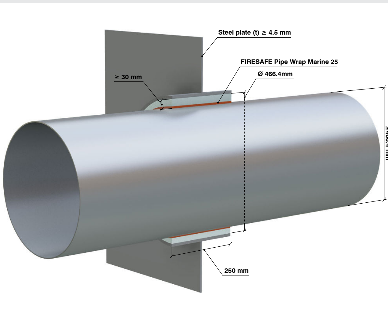
Figure 8. Thickness of GPGM 250 mm in 250 mm sleeve
