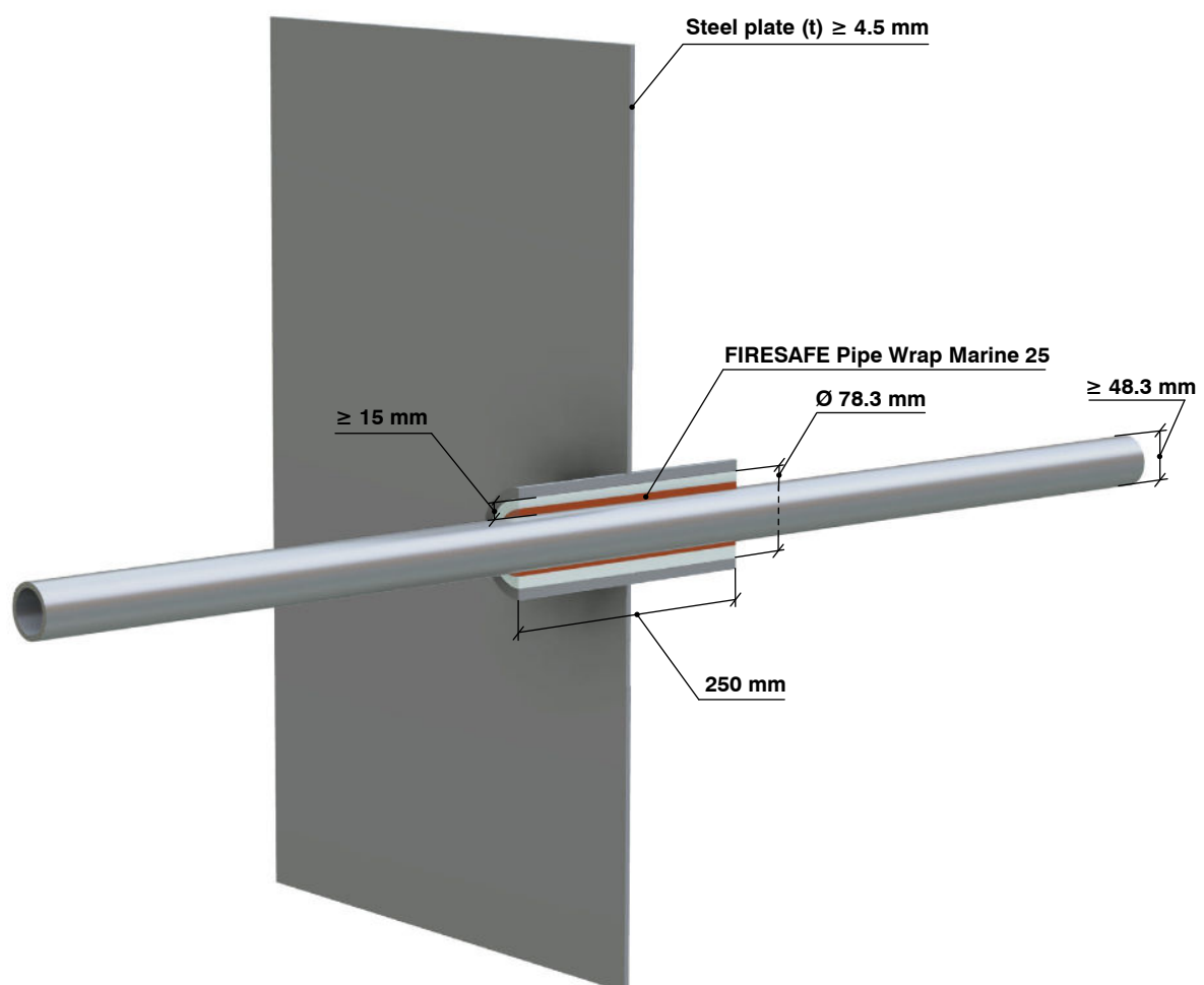
Figure 7. Thickness of GPGM 250 mm in 250 mm sleeve
