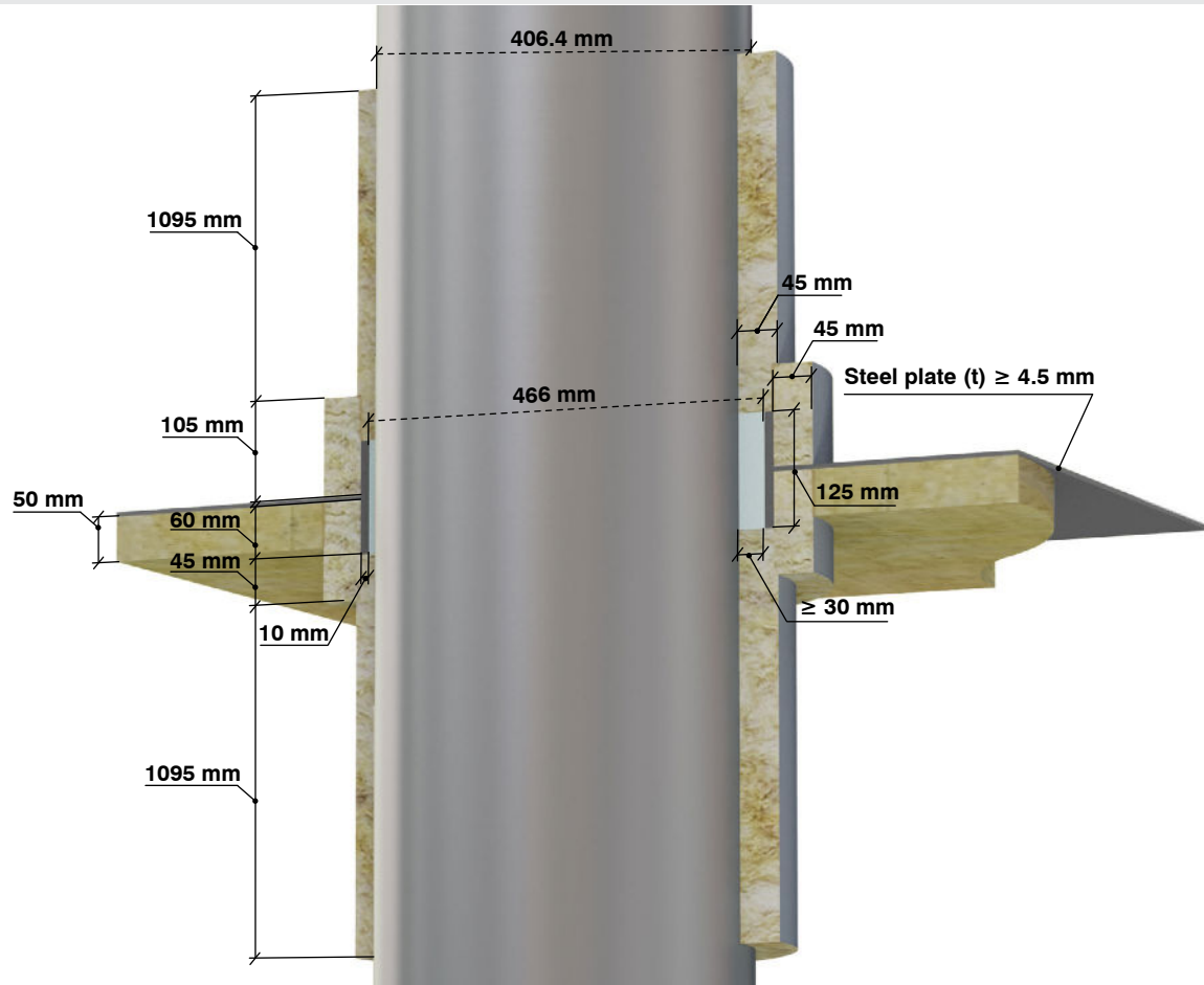
Figure 6. Thickness of GPGM 125 mm in 125 mm sleeve
