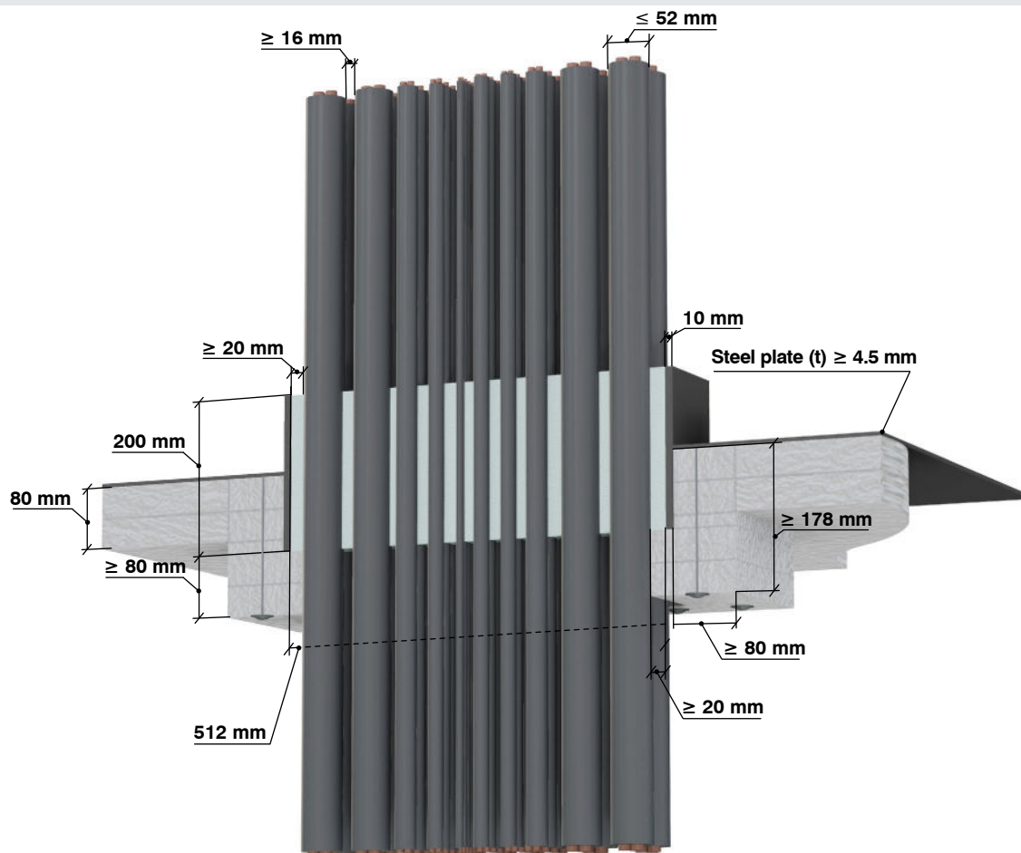
Figure 21. Thickness of GPGM 200 mm in 200 mm sleeve
