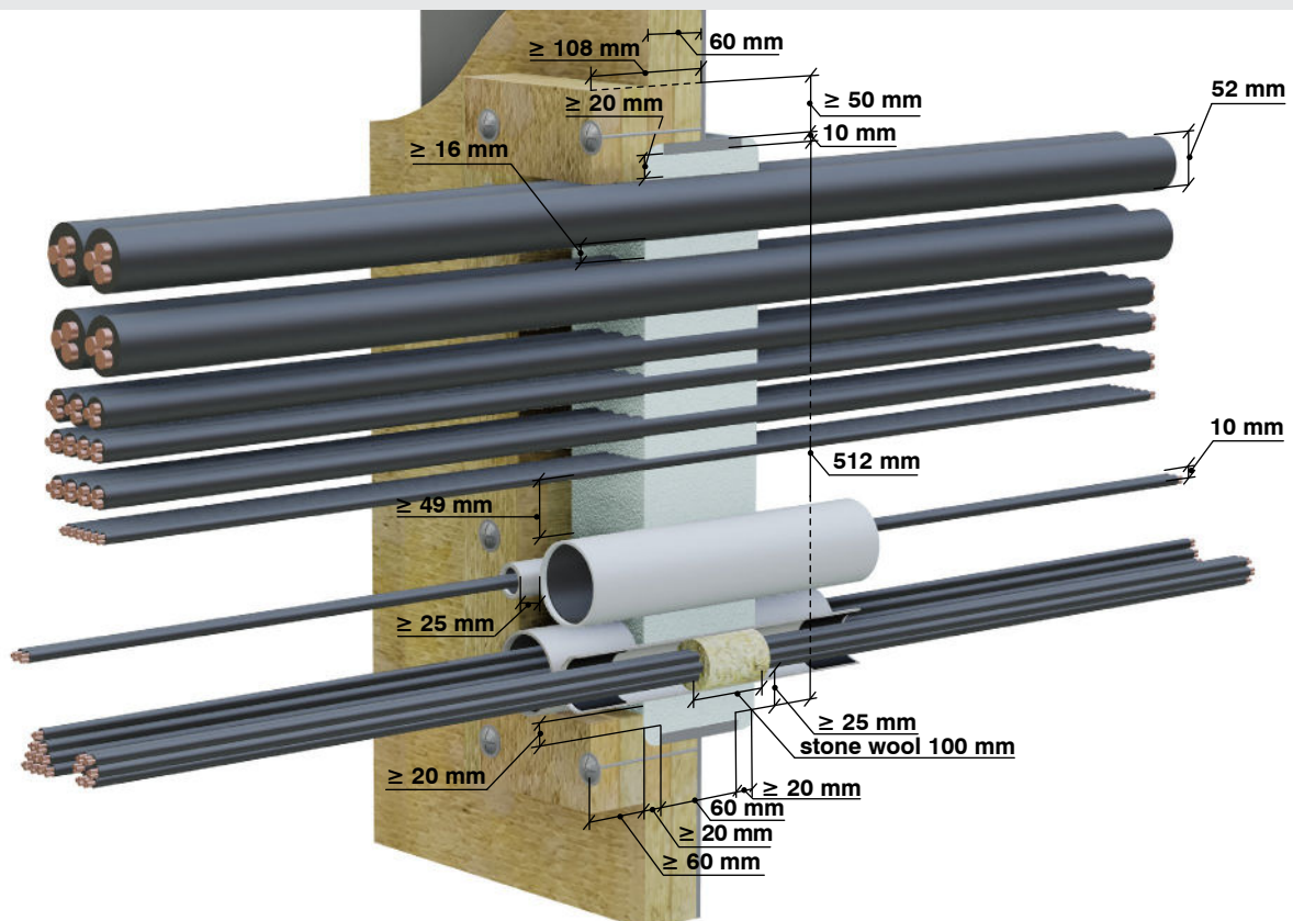
Figure 10. Thickness of GPGM 100 mm in 60 mm sleeve
